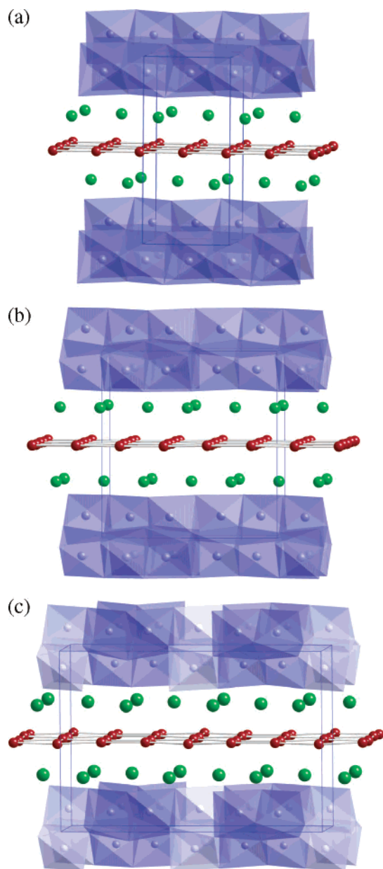
Figure 3. Polyhedral representations of the structures of (a) \text{CeCrSb}_3 , (b) \beta\text{-CeNiSb}_3 , and (c) \alpha\text{-CeNiSb}_3 viewed in the ac -plane. The green circles are Ce atoms, and the maroon circles are Sb atoms. The blue-shaded octahedra represent \text{TSb}_6 . The dark blue and light blue polyhedra distinguish the two inequivalent crystallographic Ni atom sites.
